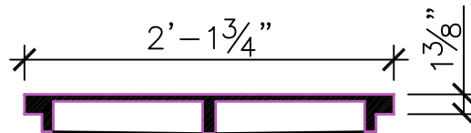
SECTION VIEW OF COVER
