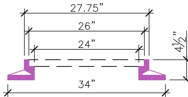
SECTION VIEW OF 4" FRAME
