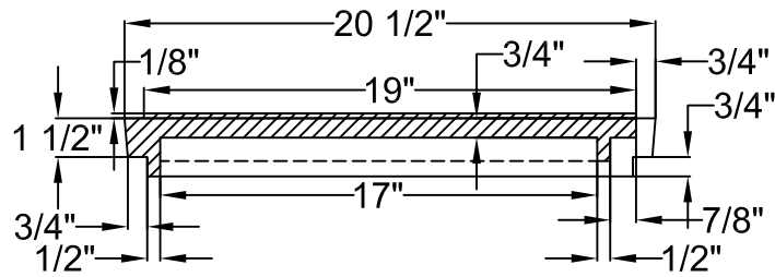
SECTION VIEW OF FRAME
