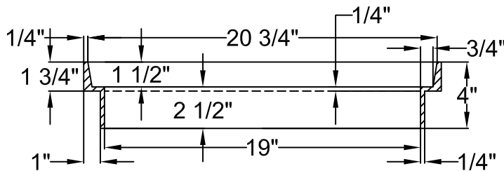
SECTION VIEW OF COVER
