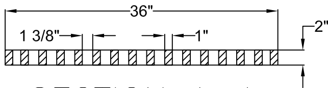
SECTION A-A OF GRATE
