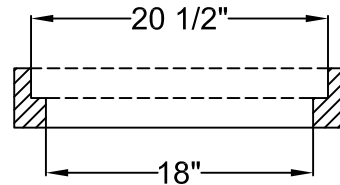
SECTION B-B OF FRAME
