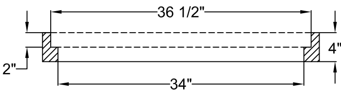
SECTION A-A OF FRAME
