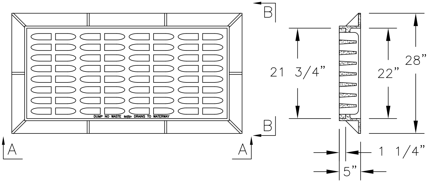
SECTION B-B
