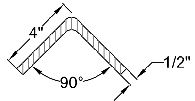
#3 REBAR DETAIL
