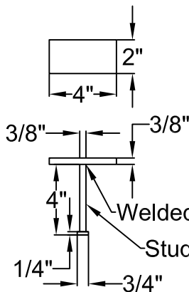
BEARING PLATE DETAIL
