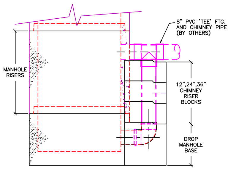
DROP MANHOLE CHIMNEY BLOCK ASSEMBLY
