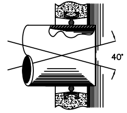
PIPE TO MANHOLE SEAL STAR-SEAL™ GASKET PER ASTM RUBBER GASKET SPECS C923, JOINT ALLOWS 20° OMNIDIRECTIONAL DEFLECTION
