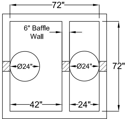
SECTION VIEW
