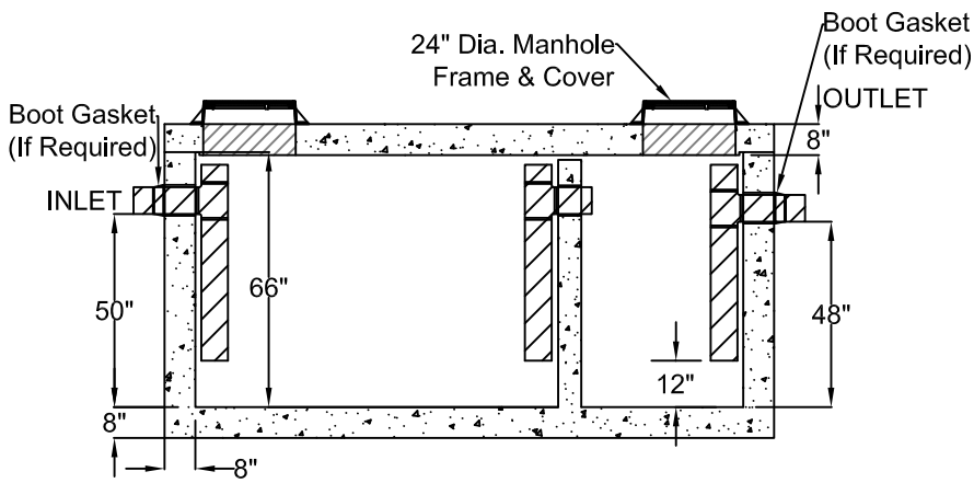
SECTION VIEW
