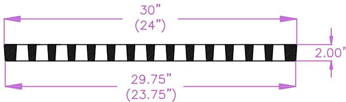
SECTION B-B
